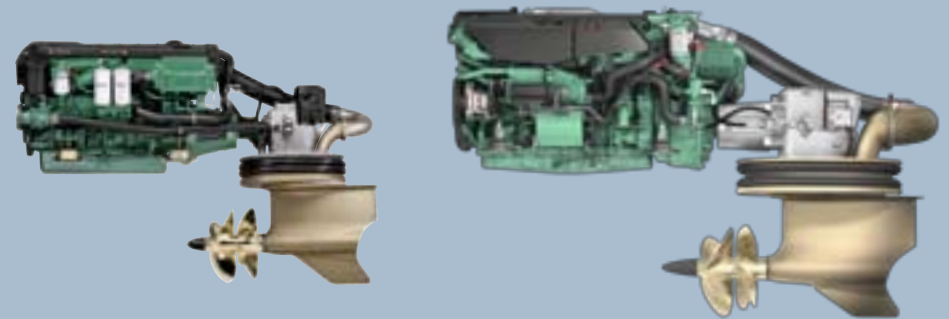
Both the IPS600 and the IPS900 are perfectly matched to their respective power and torque. With 2.5 times higher torque and 70% larger propeller blade area, the new IPS900 offers equivalent performance for yachts up to 100 feet.
